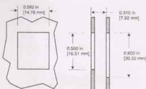
Suggested Flush Mount Panel Application Cutout
