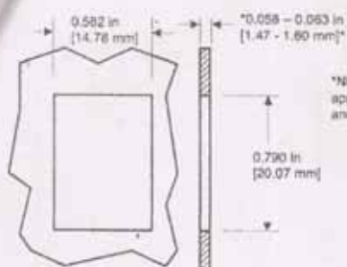
Single Panel Cutout
